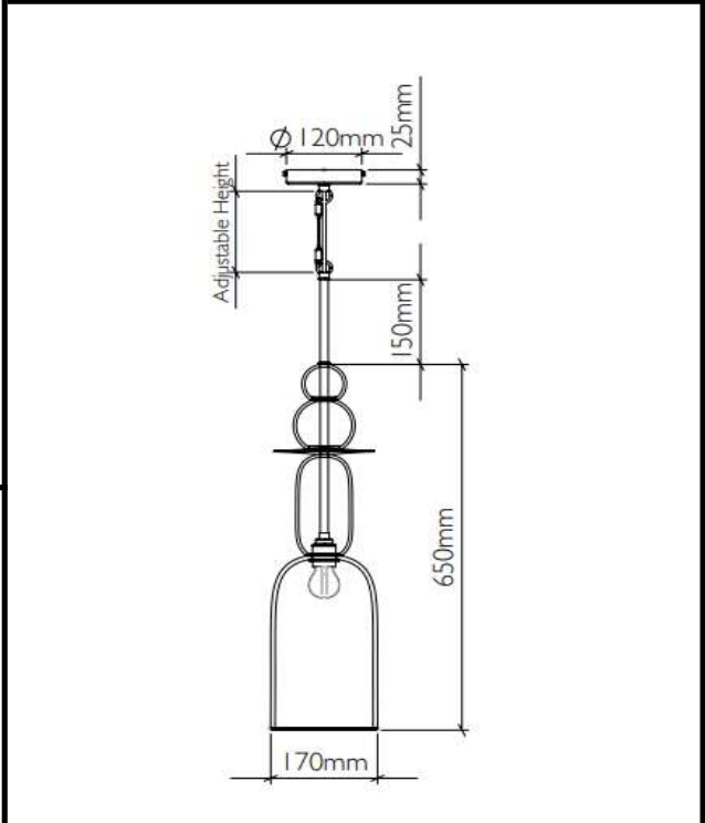
Dimension diagram
